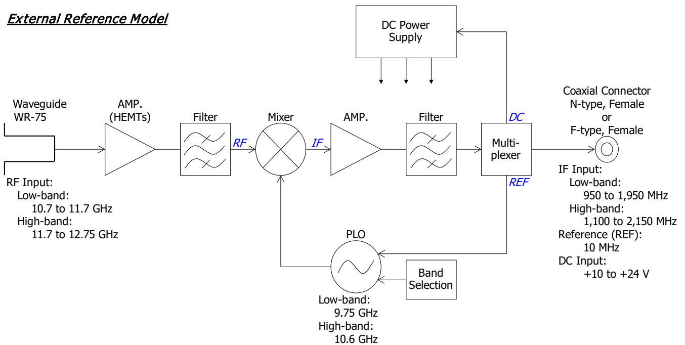
Fig.2 Functional Block Diagram
